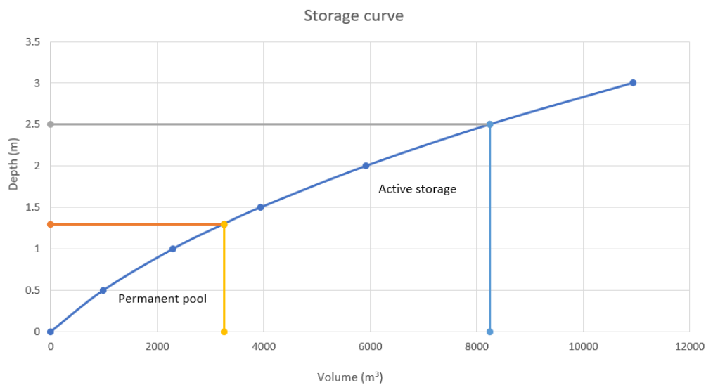
Figure 15: Storage curve
