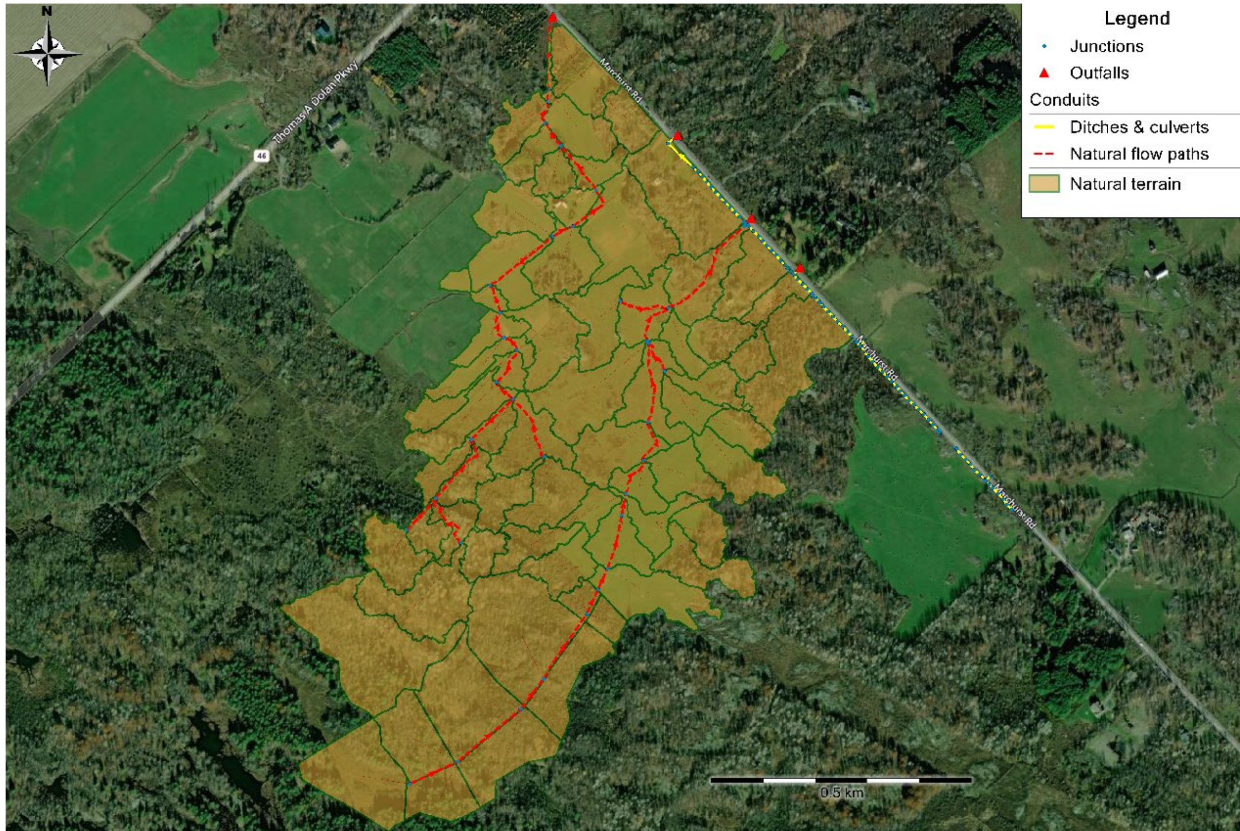
Figure 11: Pre-development sub-catchments (From PCSWMM model)
