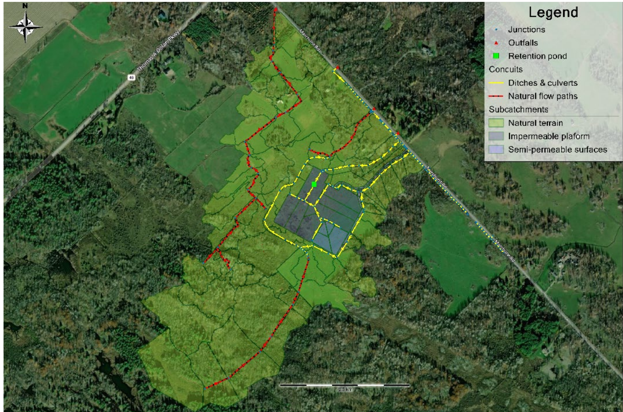
Figure 12: Post-development sub-catchment areas (from PCSWMM)
