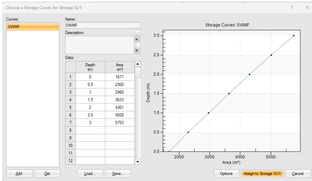
Figure 14: PCSWMM Storage curve
