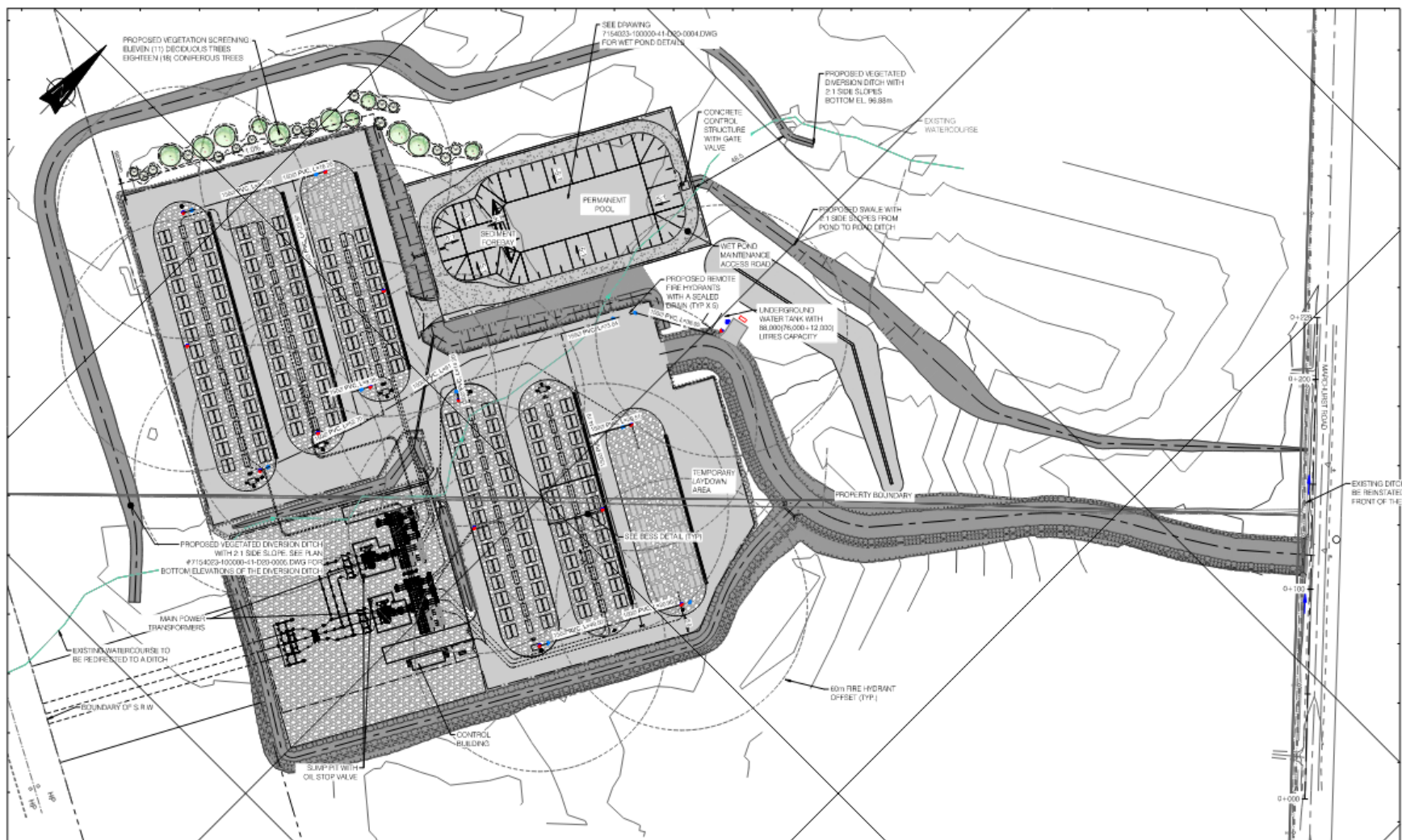
Figure 3: Watercourse path through the BESS site
